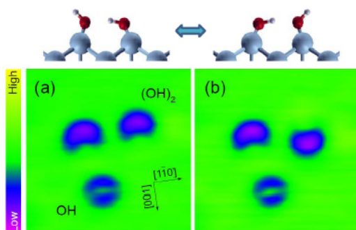
Hydroxyl switching
