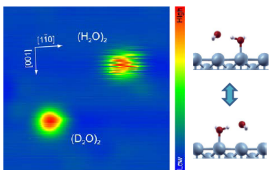
Hydrogen-bond exchange in a water dimer
