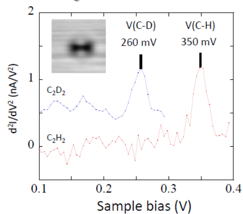
Single-molecule vibrations
