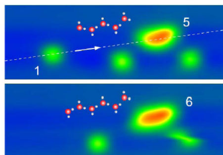
Assembling water clusters
